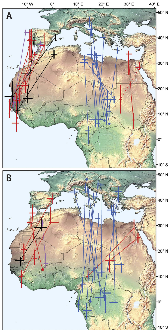
Figure 3. Autumn (A) and spring (B) stationary sites of birds (median \pm 25 th and 75 th percentiles of location estimates) just prior and after the occurrence of the full light pattern (blue = collared flycatcher, black = pied flycatcher, red = Eurasian reed warbler, purple = aquatic warbler). The two dashed lines connect stationary sites for birds without FLP. The background map was made with Natural Earth public domain free vector and raster map data@naturalearthdata.com. The stationary sites were depicted in ArcGIS.
